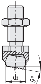
GN 709.3-R
